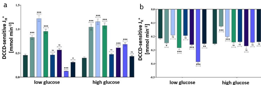
Fig 6. DCCD-sensitive J_{H^+} flux (a) and J_{K^+} flux (b) by whole cells of E. coli wild type and hyf mutants. Bacteria were grown under fermentative conditions at pH 7.5 in the presence of 2 g L -1 glucose at 37°C. During assays either 2 g L -1 (low) or 8 g L -1 (high) glucose was supplemented. DCCD (0.2 mM) was added to the assay medium when indicated. DCCD-sensitive fluxes were calculated as a difference between total and DCCD-inhibited fluxes. Positive value indicates efflux and negative value indicates influx.
